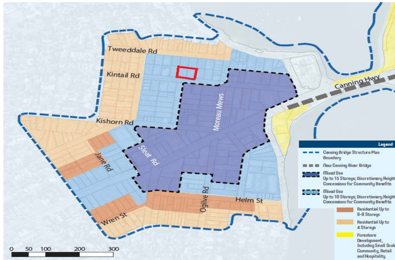
Figure 1. Canning Bridge Structure Plan Land Use, Built Form and Zones
