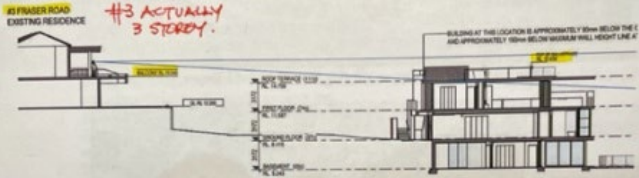
Figure 5: Cross- Sections
