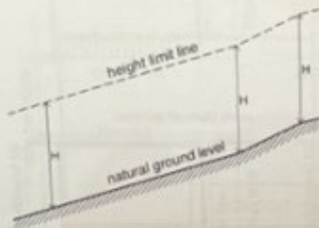
Figure 7a – Measuring building height
