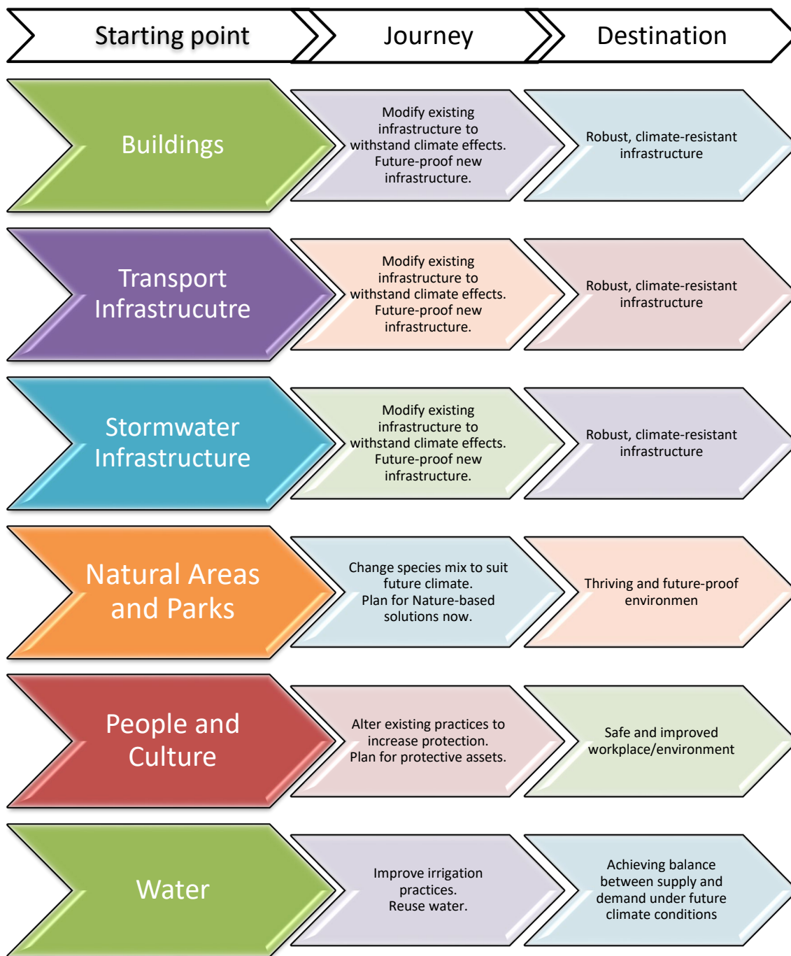
Figure 10 Adaptation guide.
