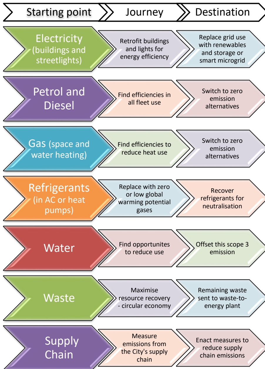
Figure 9 Mitigation Guide.
