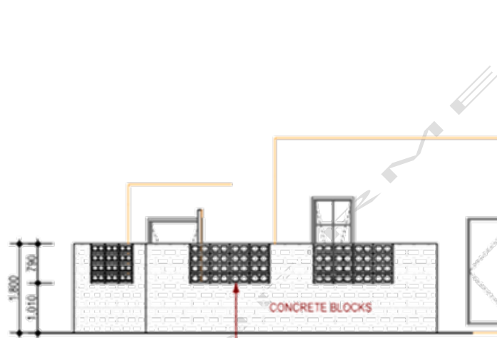
FENCE ELEVATION 1:100
