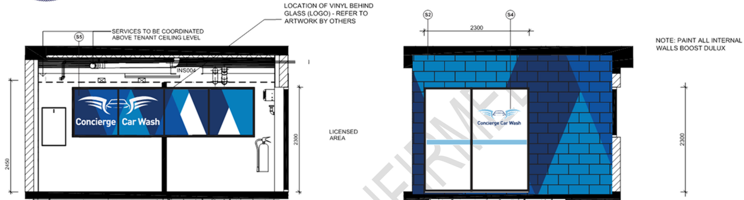
01 Elevation - CONCIERGE CARWASH - SCALE 1:50
