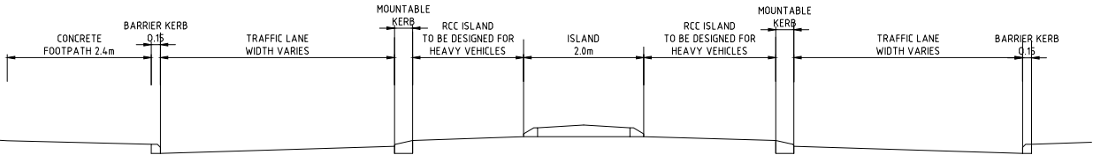
TYPICAL CROSS SECTION SCALE NTS
