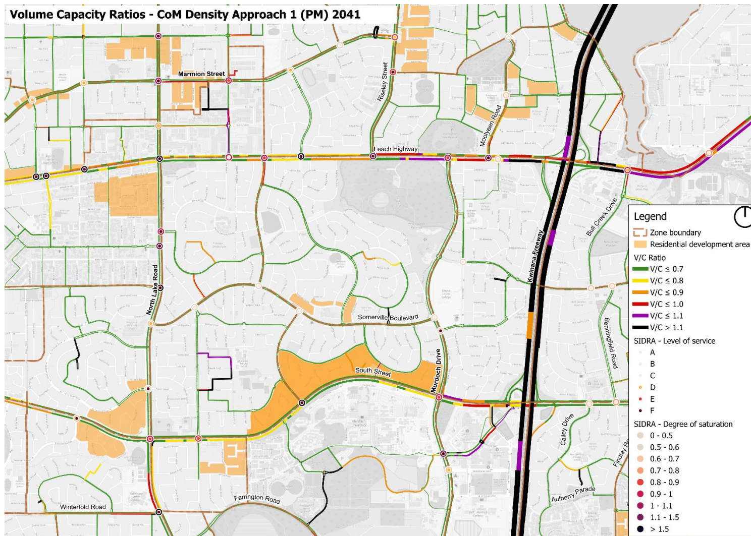
Figure C.29 Existing network volume-capacity ratios and intersection performance– 2041 scenario 1 PM (“CoM Density Approach 1”) (zoomed, Leach Highway and South Street)
