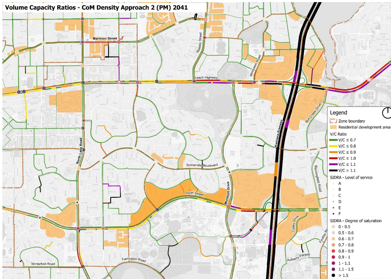
Figure C.39 Existing network volume-capacity ratios and intersection performance– 2041 scenario 2 PM (“CoM Density Approach 2”) (zoomed, Leach Highway and South Street)
