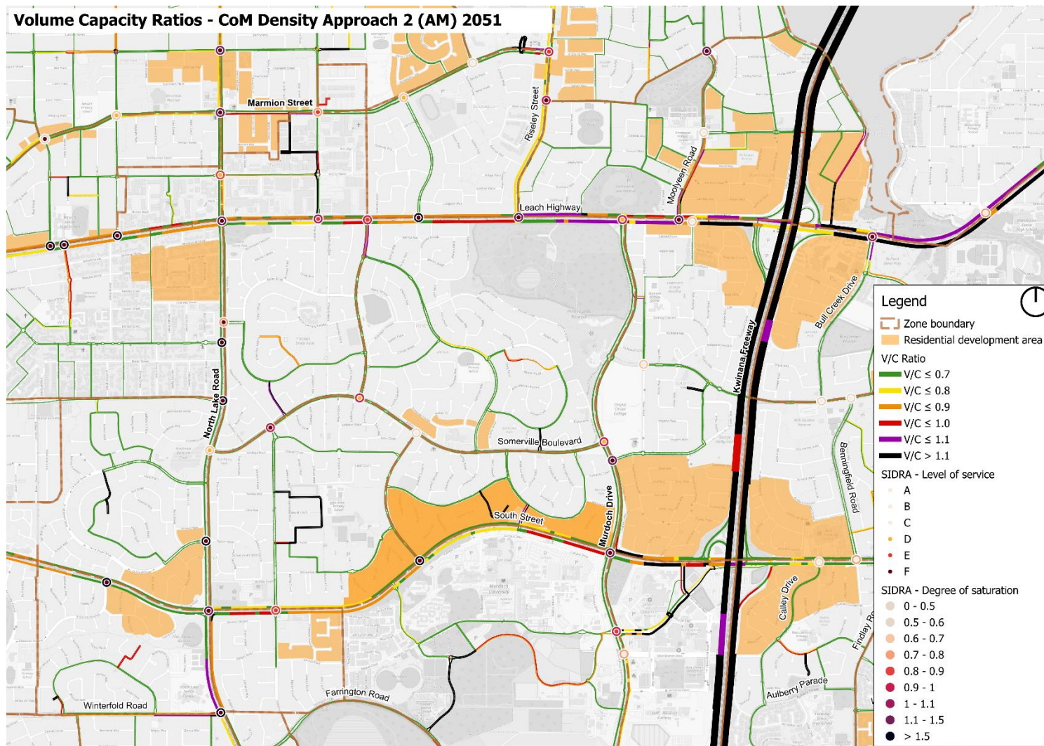
Figure C.64 Existing network volume-capacity ratios and intersection performance– 2051 scenario 2 AM (“CoM Density Approach 2”) (zoomed, Leach Highway and South Street)
