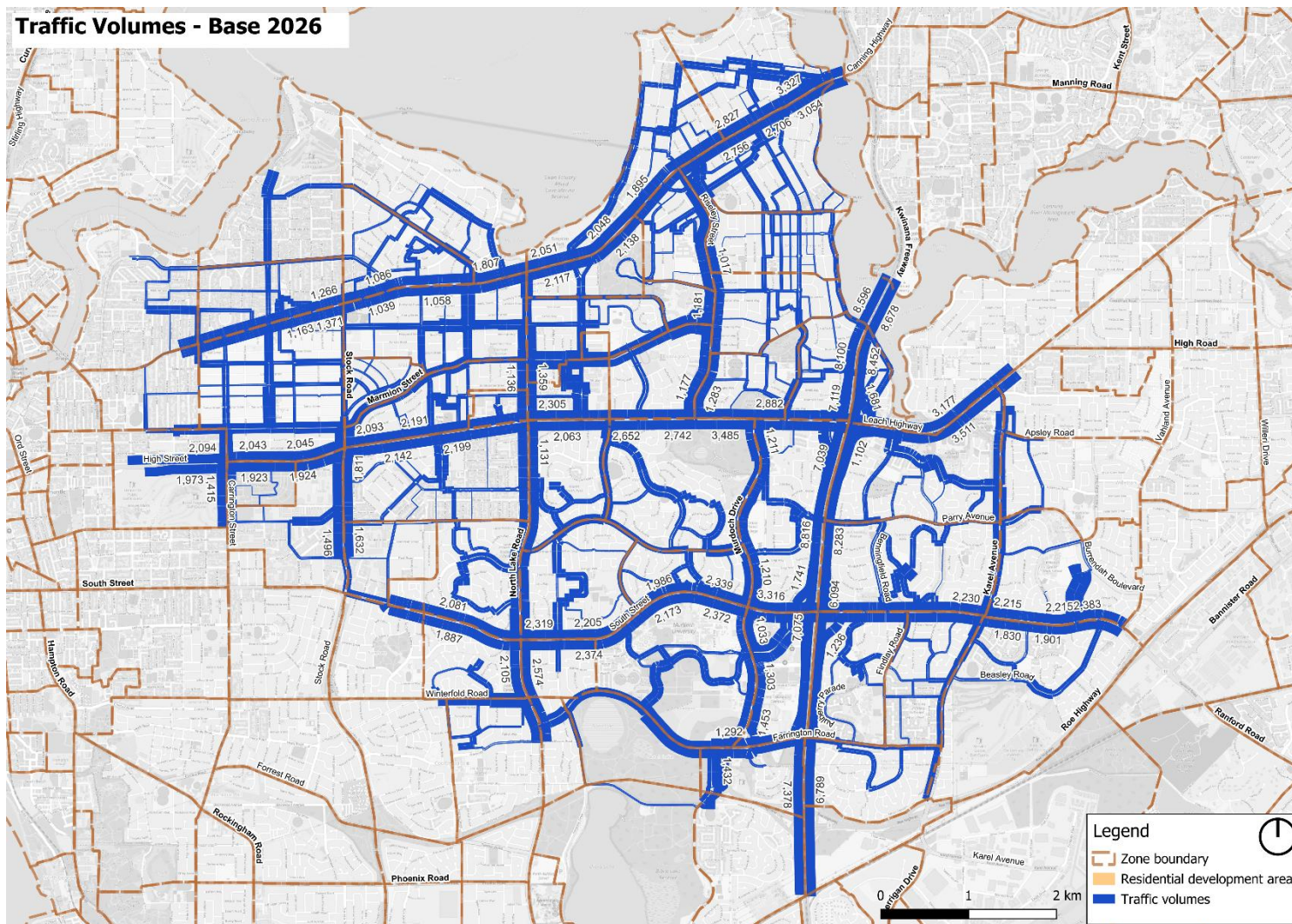
Figure A.1 Existing network flows – 2026 Base
