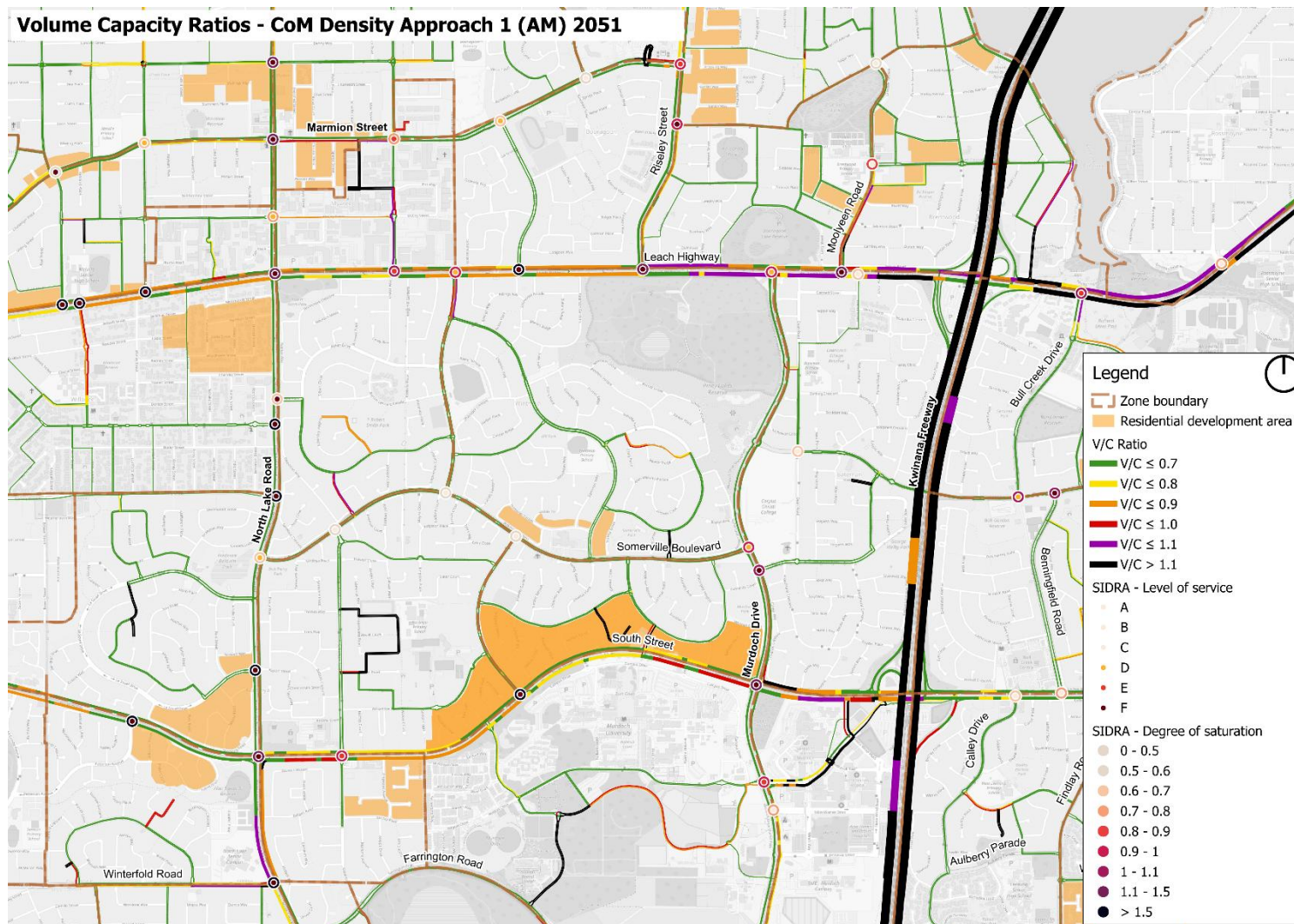
Figure C.54 Existing network volume-capacity ratios and intersection performance– 2051 scenario 1 AM (“CoM Density Approach 1”) (zoomed, Leach Highway and South Street)
