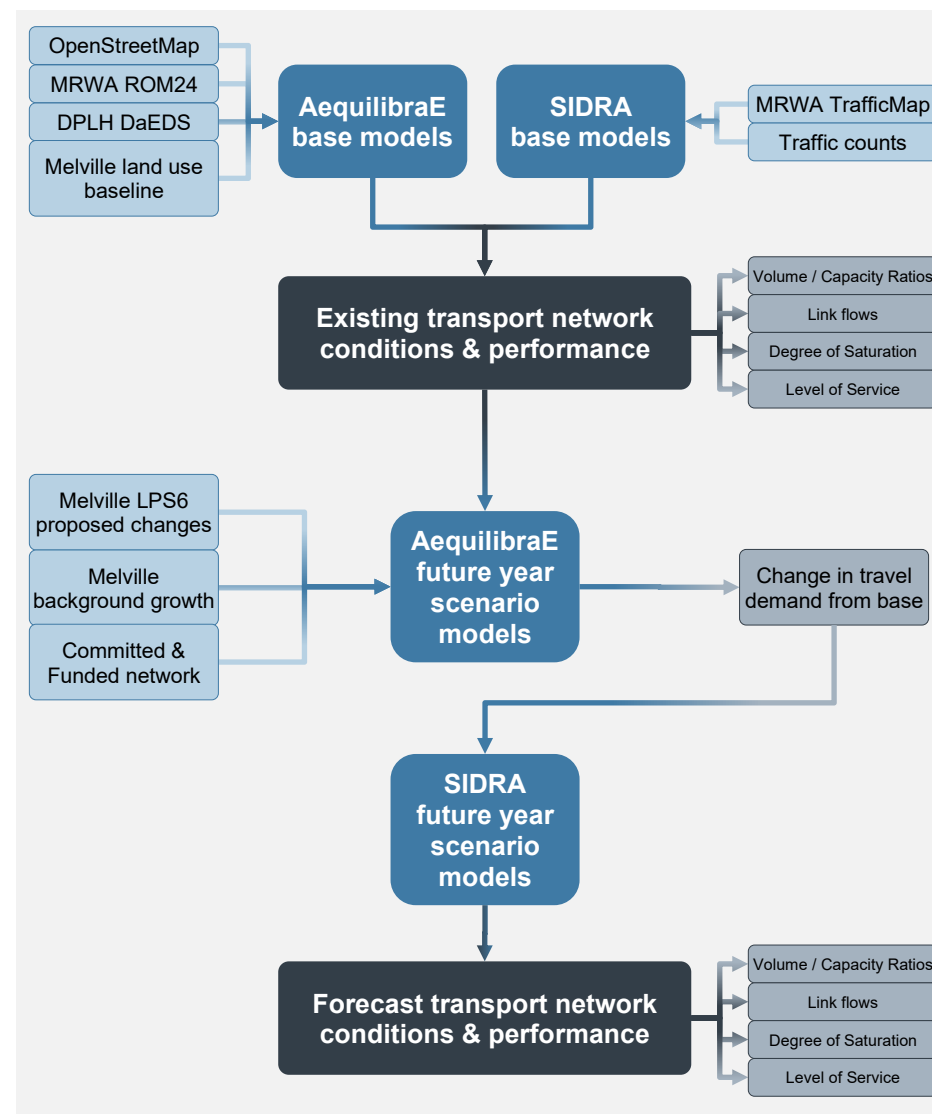
Figure 4.1 High-level transport network assessment methodology
