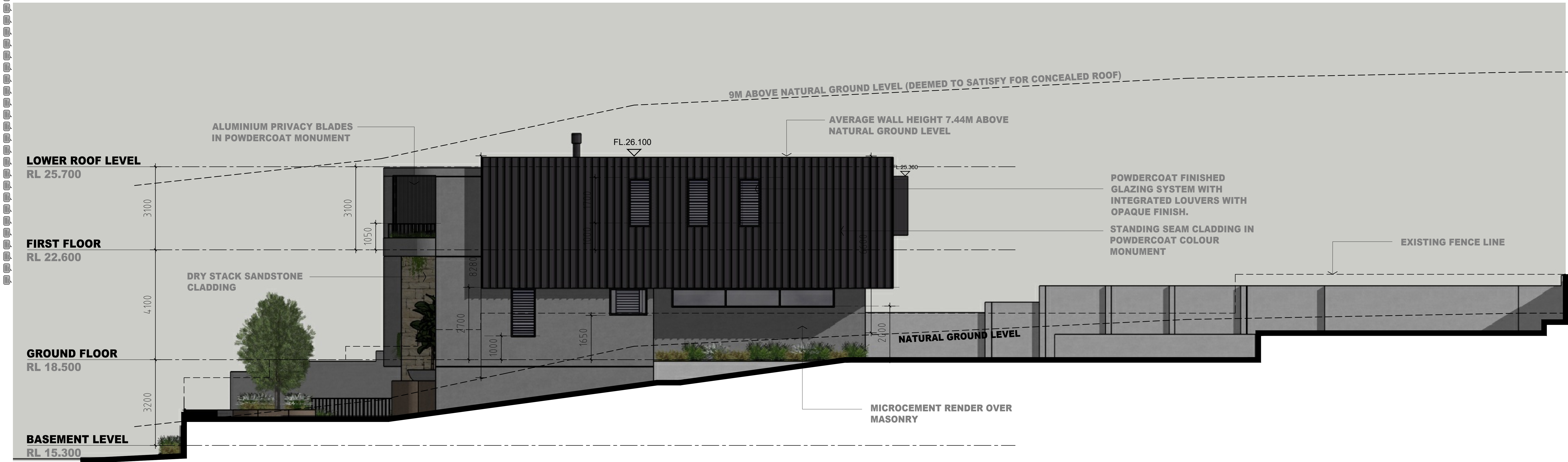
NORTH ELEVATION SCALE 1:50 @ A0
