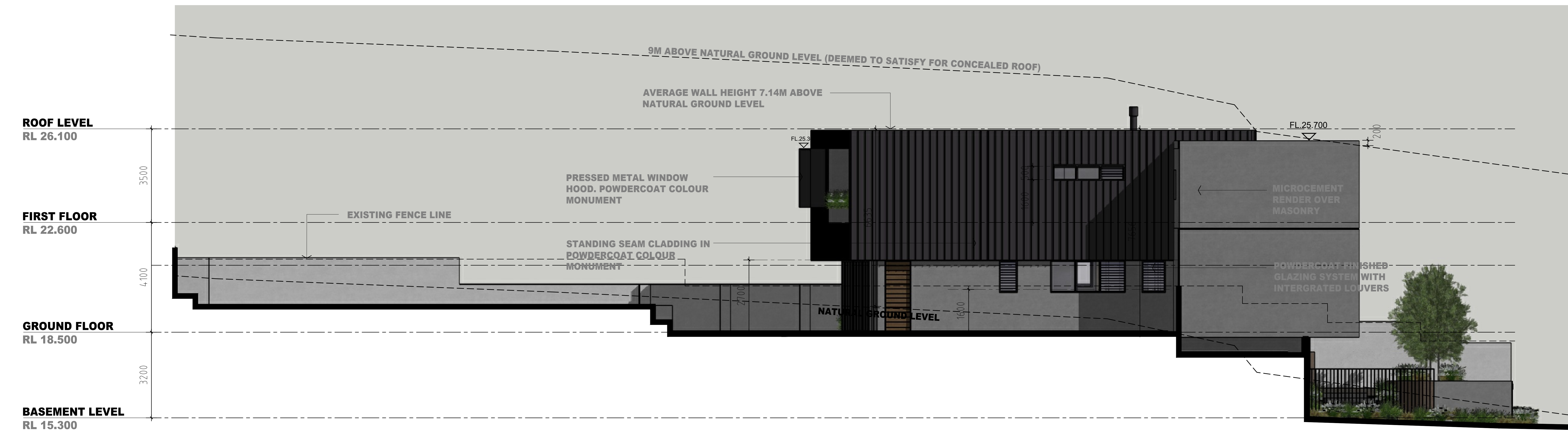
SOUTH ELEVATION SCALE 1:50 @ A0
