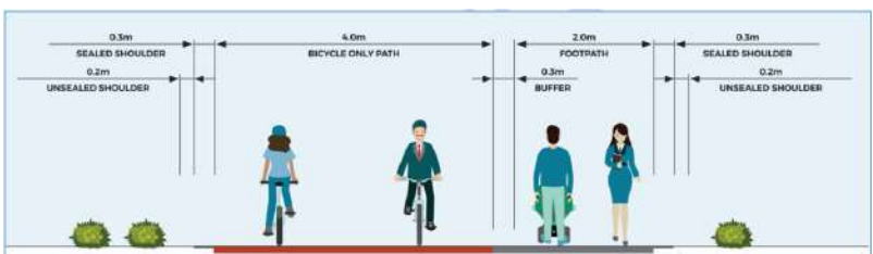
Pedestrian and cyclist separation
